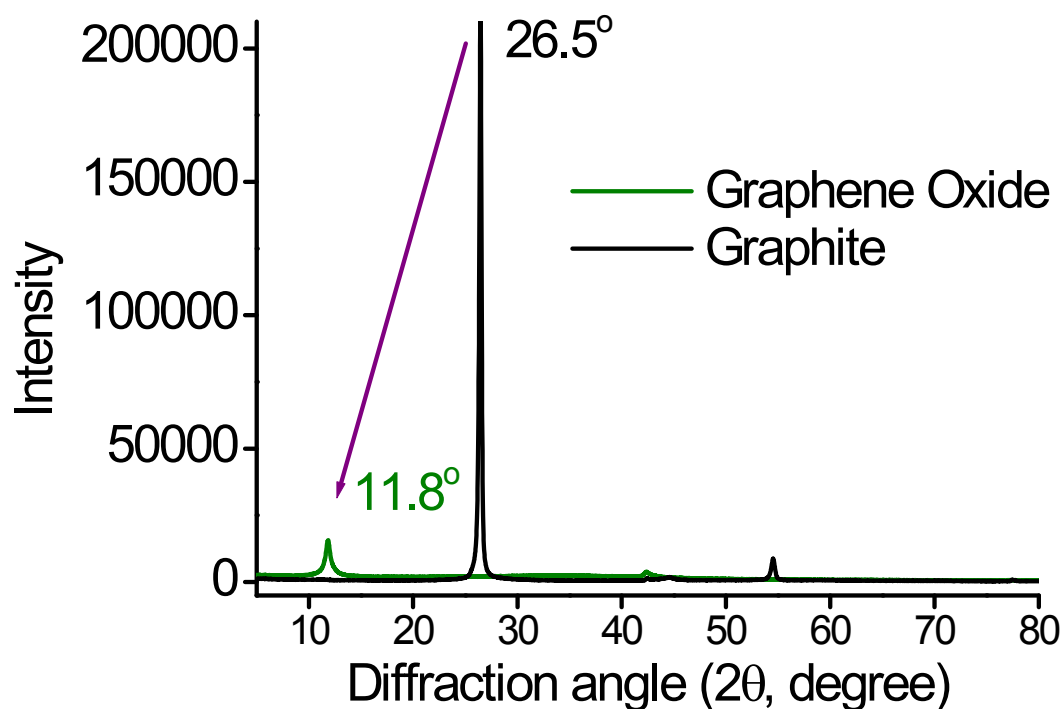
Fig. S1. XRD patterns of graphite and graphene oxide.
