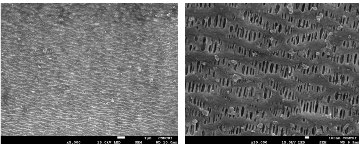
Figure S1: FE-SEM images of recovered separators (PP and PE) from spent LIBs (Random sampling).
