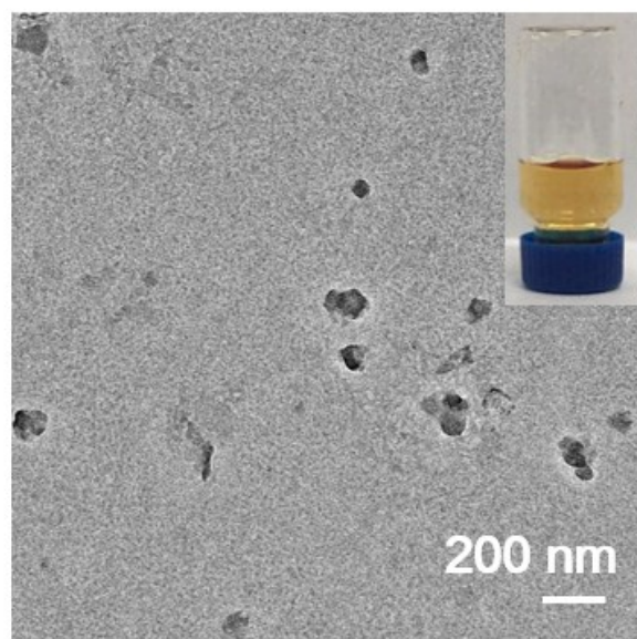
Figure S2. TEM image of C 60 -PTC aggregates in aqueous solution aged for 1 day (inset is the photograph of the solution).
