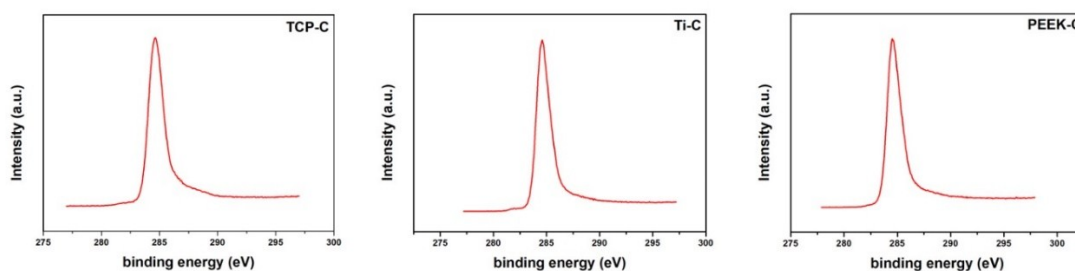
Fig. S2 XPS spectra of the TCP-C, Ti-C and PEEK-C samples.
