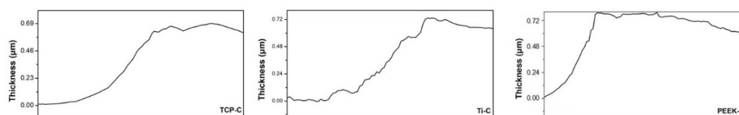
Fig. S1 The thickness of carbon-coating measured by AFM.
