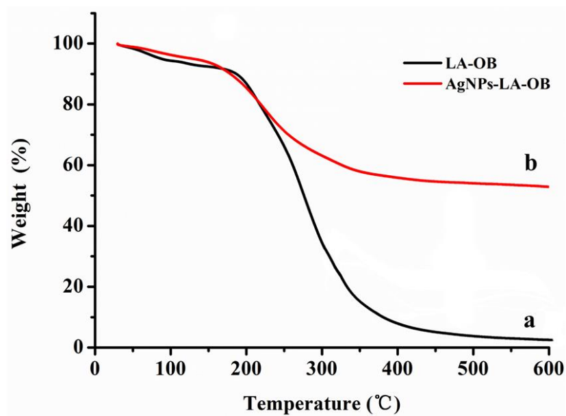
Figure S1. TGA curves of LA-OB (a) and AgNPs-LA-OB (b)
