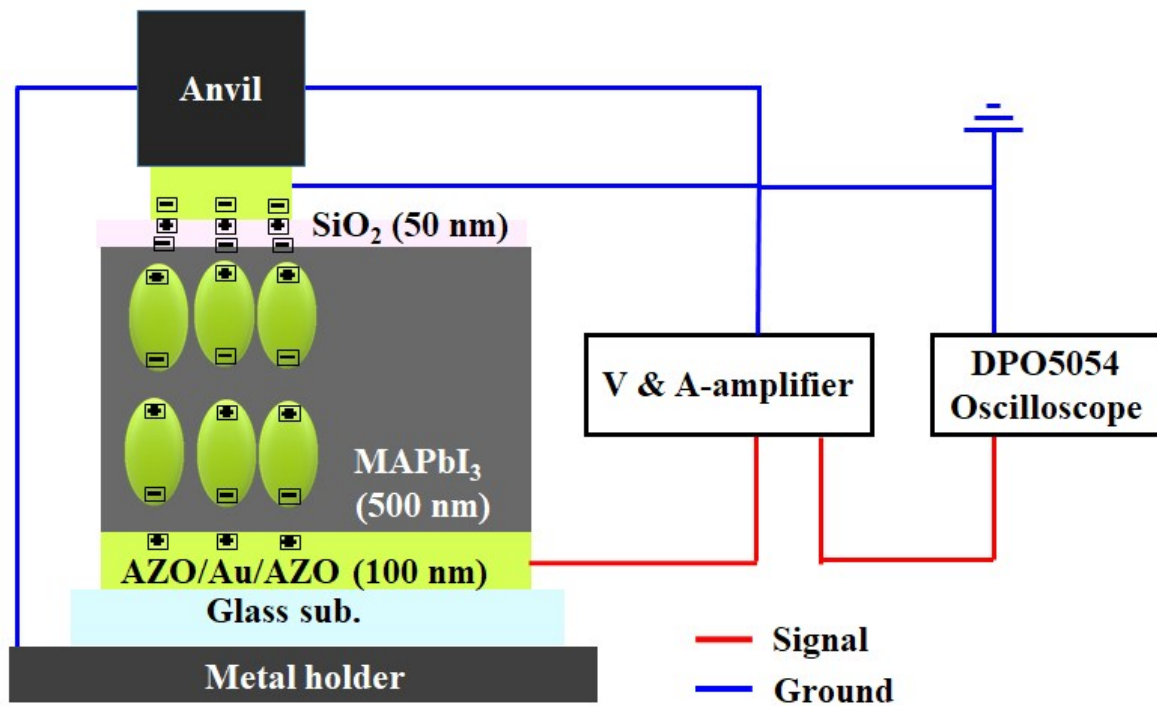
Fig. S1 Schematic structure of electric circuit to remove the triboelectric effect of the piezoelectric sensors.
