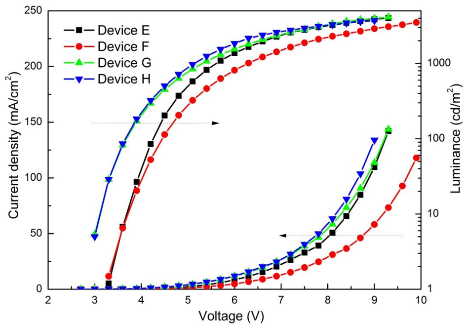
Fig. S2 The current density-voltage-luminance curves of Device E to Device H.
