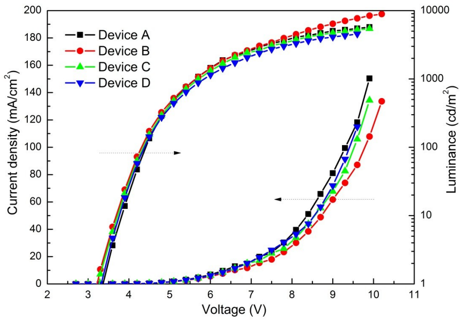
Fig. S1 The current density-voltage-luminance curves of Device A to Device D.
