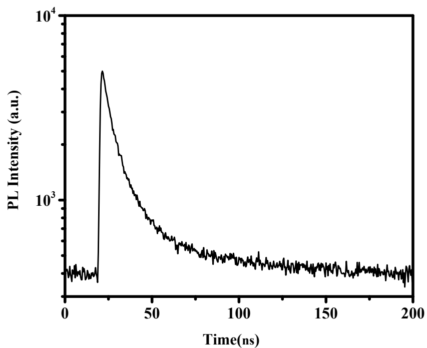
Figure S3. Transient PL decay curves of 10 wt% 4t-BuCzTTR doped CBP films in range of 200 ns. (Excitation wavelength was 300 nm.)
