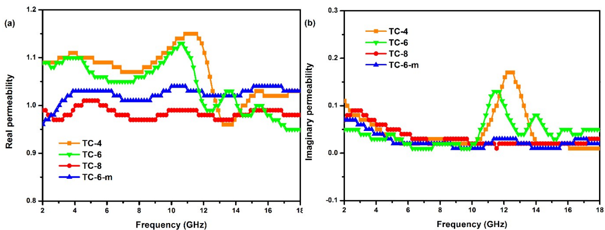
Figure S1. (a) Real part and (b) imaginary part of the related permeability spectra of the samples in the range of 2-18 GHz.
