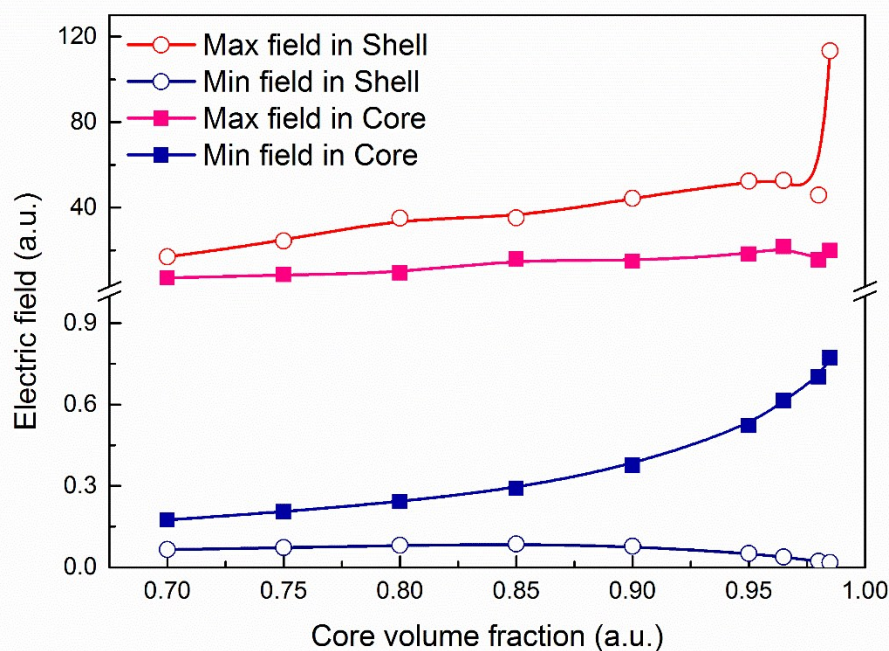
Fig. S1 Maximum and minimum electric for the core and shell material.
