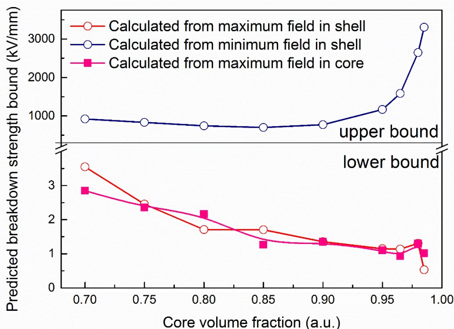
Fig. S2 Predicted bounds for the composite breakdown strength based upon the maximum and minimum electric field strength respectively found in the core and shell material.
