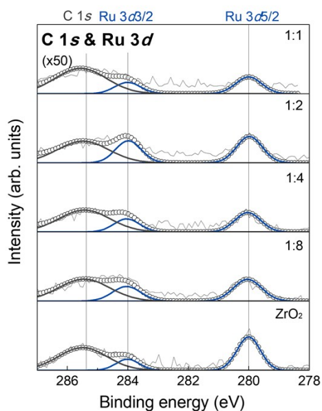
Figure S1. Ru 3d spectra of 10-nm ALD undoped and Ta-doped ZrO 2 on Ru
