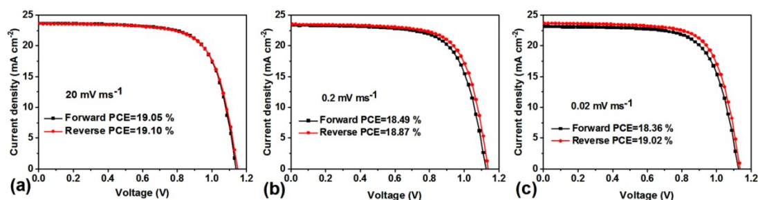
Fig. S2. J-V curves by forward and reverse scans with different rates from 0.02 to 20 mV ms -1 (the data with 2 mV ms -1 are presented in Fig. 7a in the paper).
