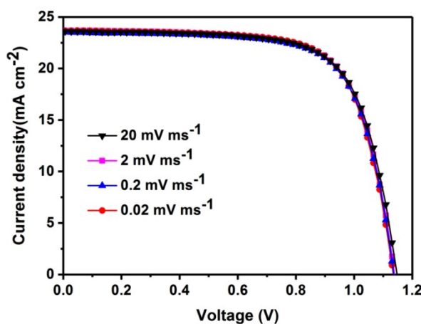
Fig. S1. J-V curves by reverse scan with different rates from 0.02 to 20 mV ms -1 .
