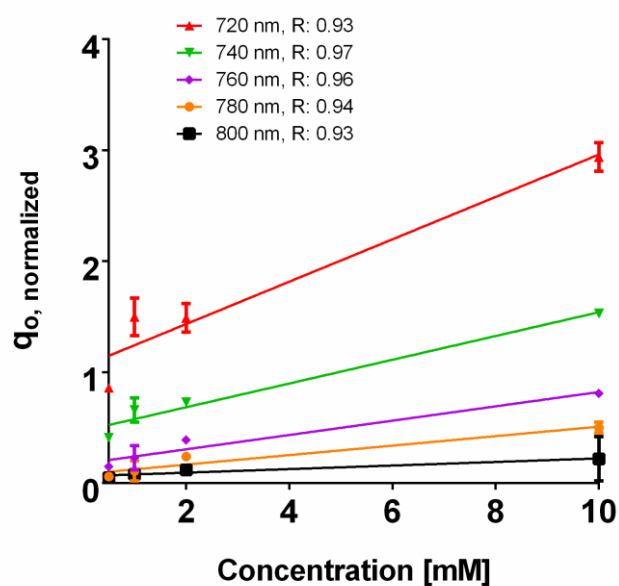
Figure S2. Concentration dependence of q_0 value to the concentration of TPP.
