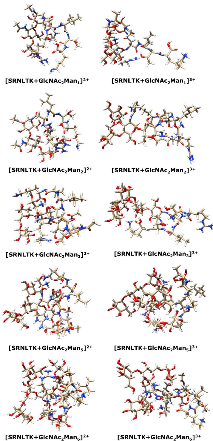
Figure S1. Energy-minimized gas-phase structures of the SRNLTK + GlcNAc 2 Man 1-3,5,6 (top to bottom) with z = 2+ (left column) and z = 3+ (right column).
