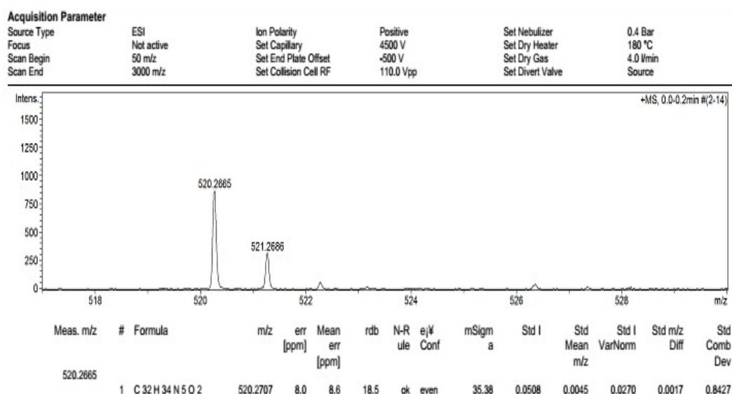
Fig. S1 HRMS of J1
