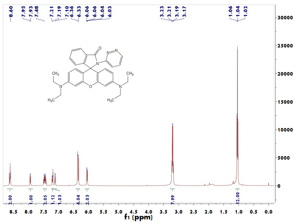
Fig. S3 1 H NMR of J1
