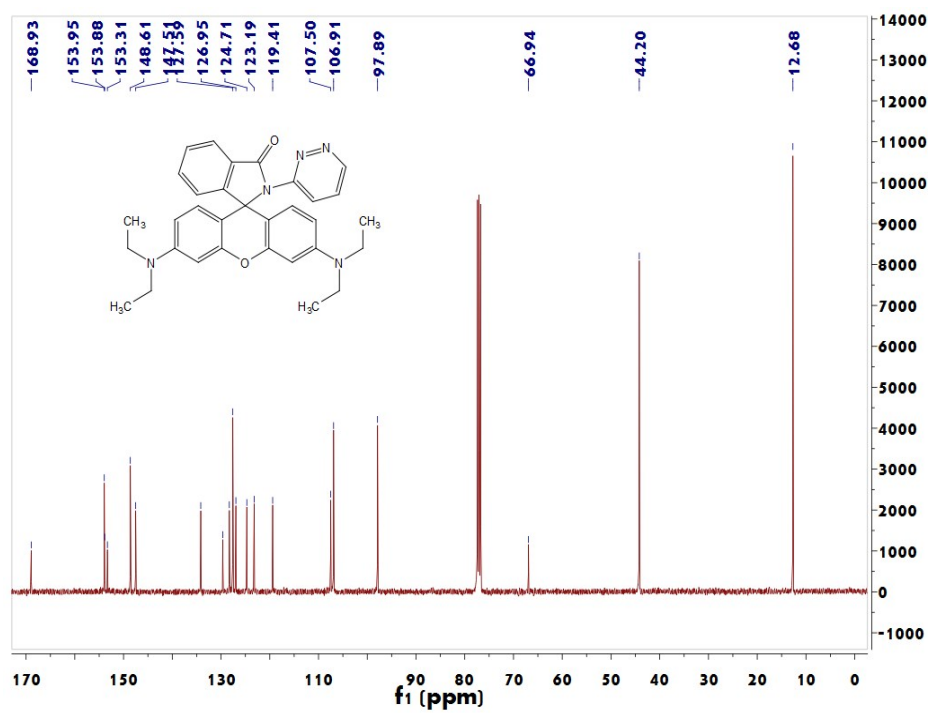
Fig. S4 ^{13}\text{C} NMR of J1
