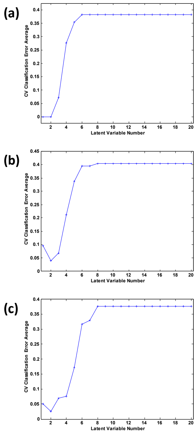
Fig. S2. Latent variable number vs CV classification error average plots for the built PLS-DA models of: (a) cranberry vs raspberry, (b) cranberry vs blueberry, and (c) cranberry vs grape.
