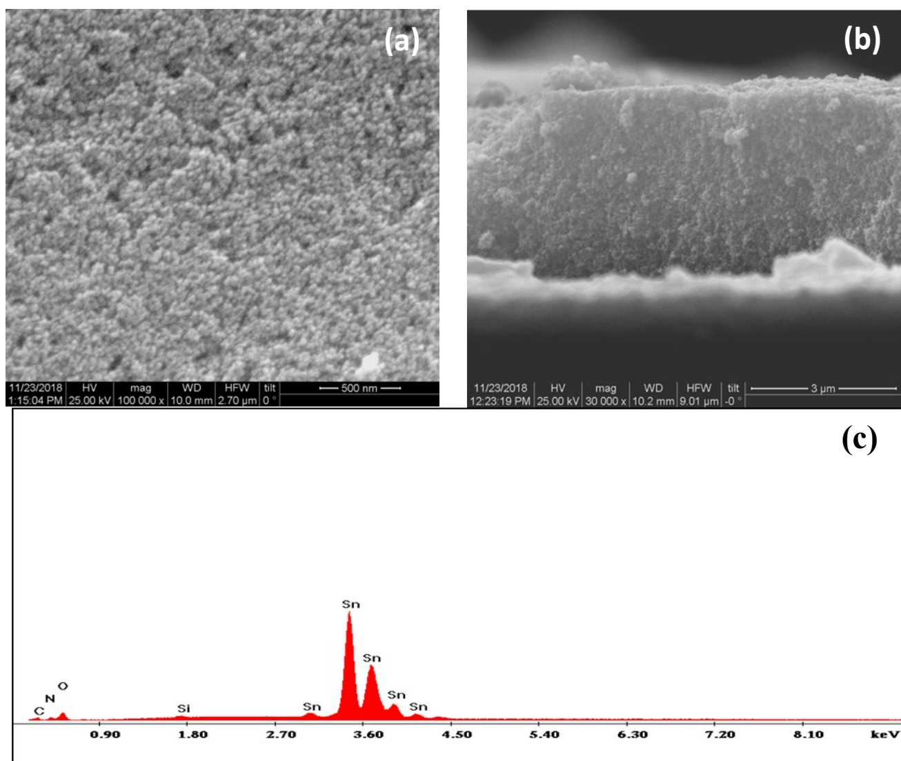
Figure S1: FE-SEM images of SnO 2 /ITO glass (a) top view, (b) side view and (c) EDS analysis.
