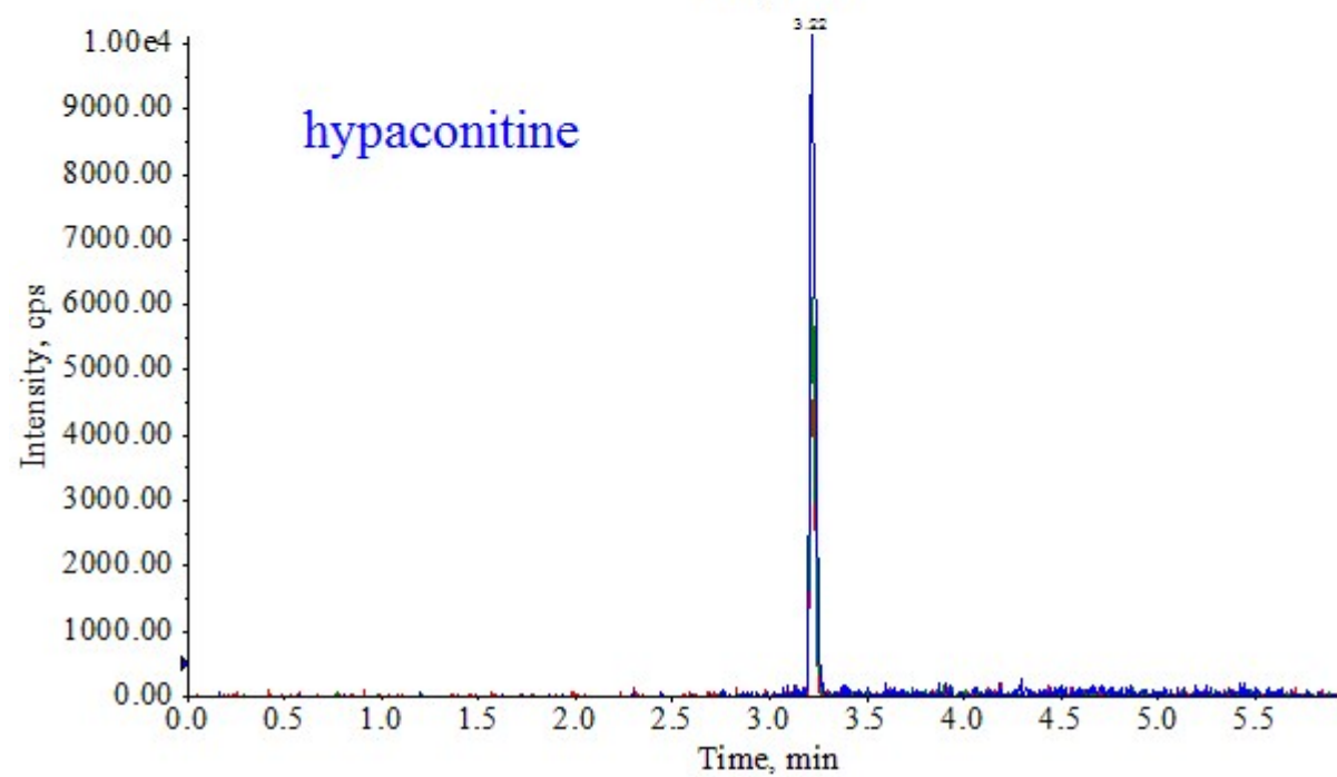
Fig. S2 The MRM chromatograms for one typical sample
