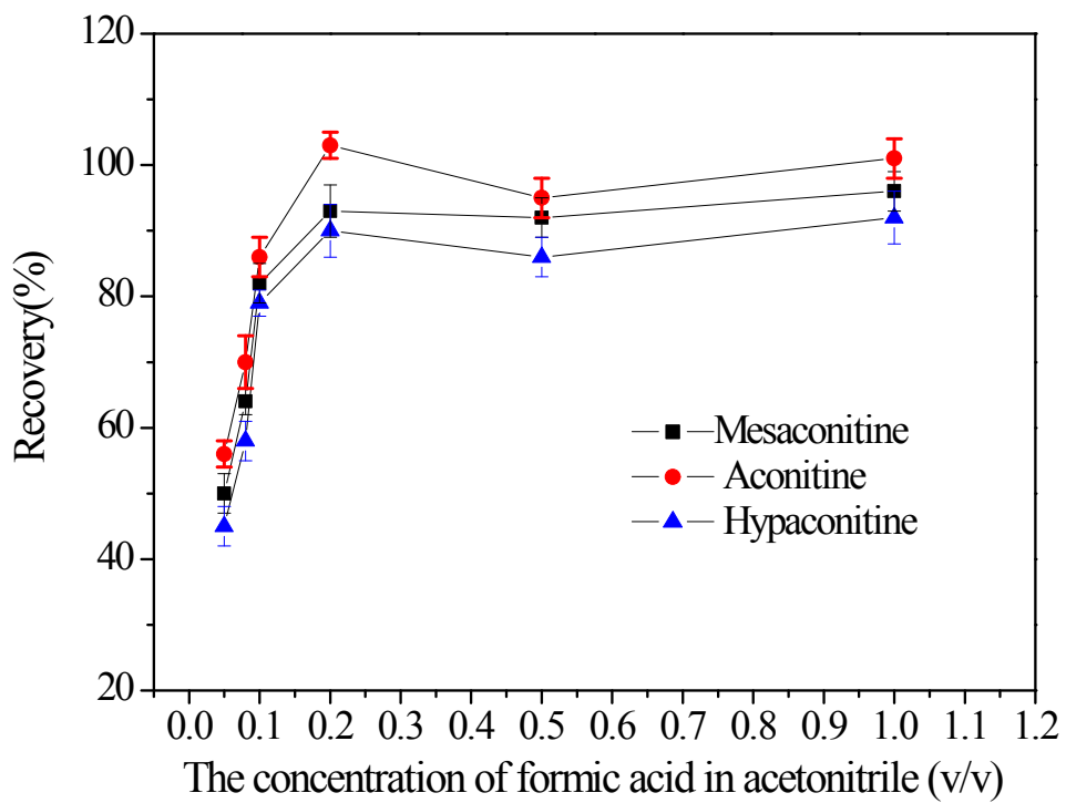
Fig. S1 Effect of the concentration of formic acid in acetonitrile on the recoveries of 3 aconitum alkaloids
