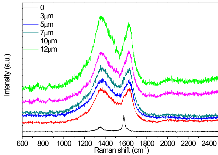
Fig.S5 Raman spectra of OMC700 fibers with different thickness
