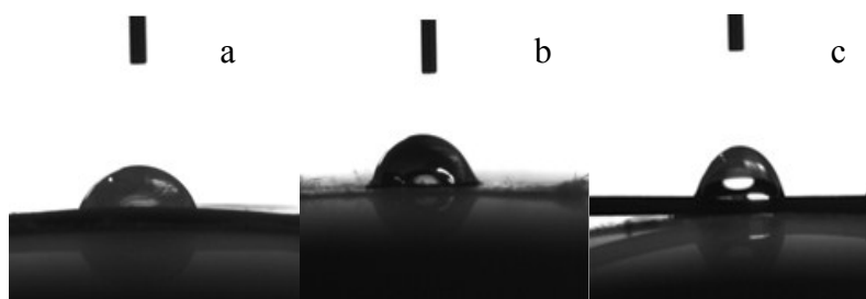
Fig.S4 Contact angle of the OMC (a: 350 °C b: 550 °C c: 700 °C)
