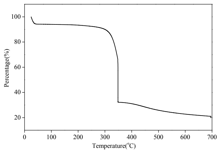
Fig.S2 TGA curve of the as-prepared OMC before calcination
