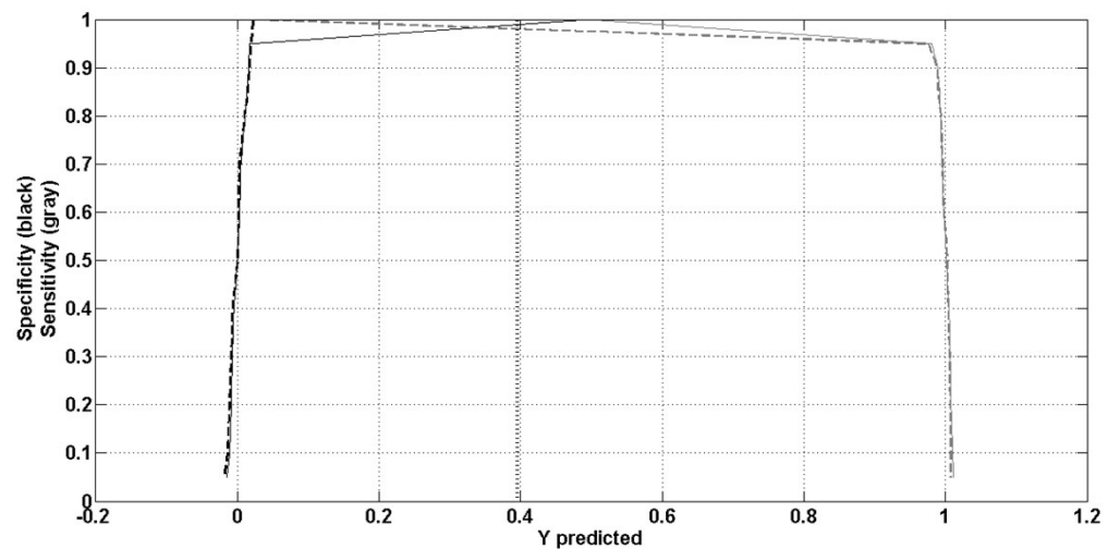
Figure 1S. ROC curve for organic sugar crystal. Solid lines correspond to the predicted values from PLS-DA model. Dashed lines correspond to the cross-validation predicted values (contiguous block of 5 samples). The vertical pointed black bold line corresponds to the threshold value of 0.3953.
