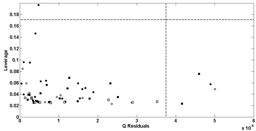
Figure 2S. Q residuals against leverage for the crystal sugar PLS-DA model. (●) organic samples in training (○) organic samples in validation. (■) conventional samples in training. (□) conventional samples in validation.
