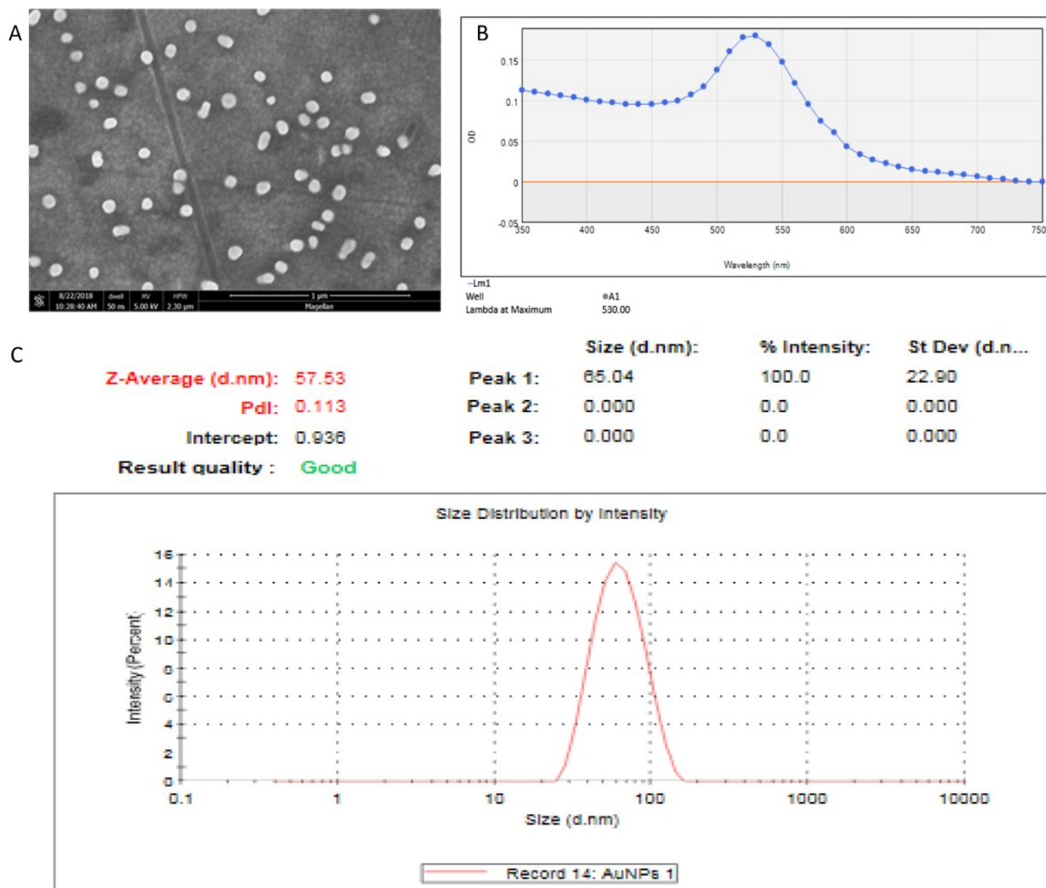
Figure 1. (A) TEM photo of home-made AuNPs, (B) UV-vis spectra of AuNPs, (C) DLS spectra of AuNPs
