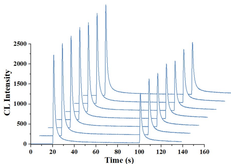
Figure S2 Repeatability analysis for the detection of β-agonists (1.0×10 -6 mol/L) on the μPAD CL sensor.
