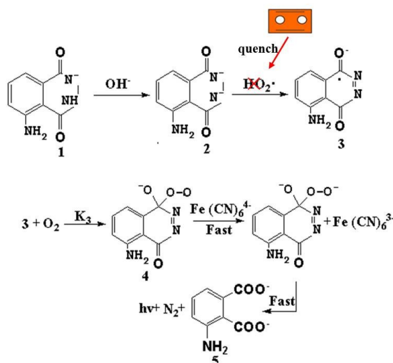
Figure S1 Schematic reaction of the CL diminishment mechanism on the μPAD.
