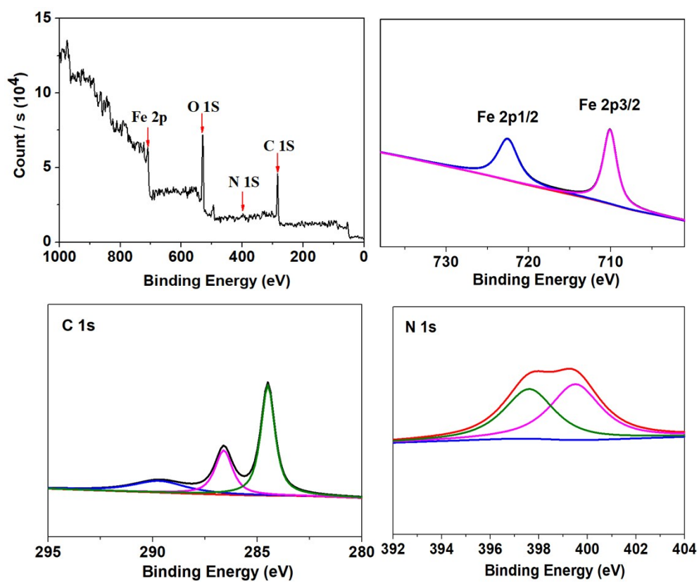
Figure S2 XPS spectra of SPIONs (a), Fe 2p (b), C 1s (c), N 1s (d).
