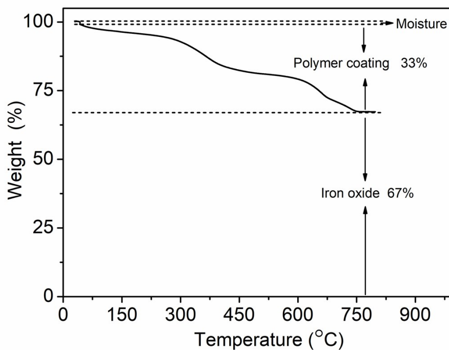
Figure S1 Thermogravimetric analyses curve of SPIONs from 0 to 800 °C.
