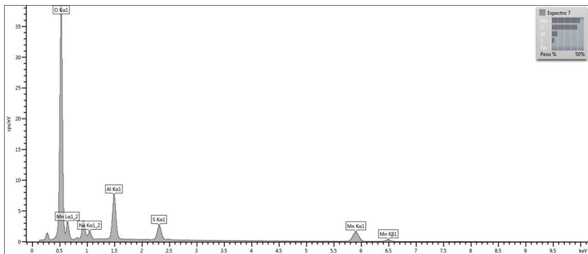
SM5 – EDS spectrum Mn/Al-CO 3 .
