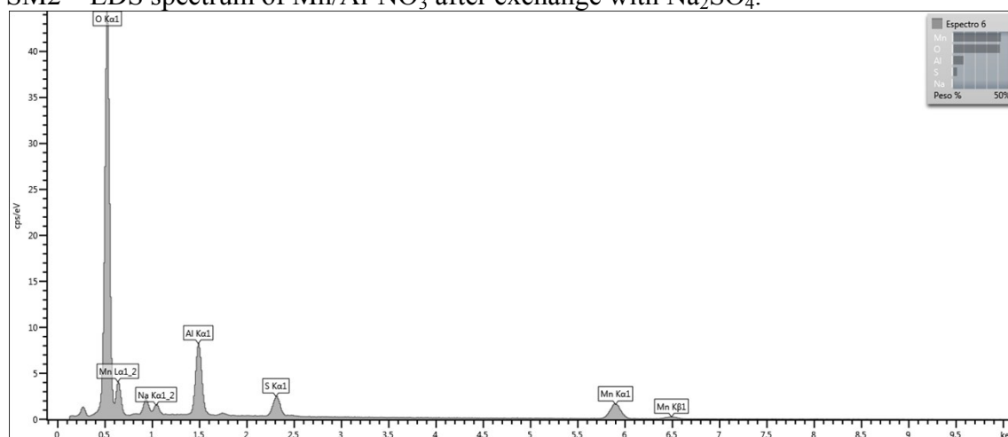
SM2 – EDS spectrum of Mn/Al-NO 3 after exchange with Na 2 SO 4 .
