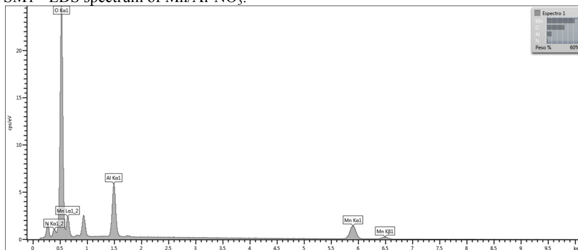
SM1 - EDS spectrum of Mn/Al-NO 3 .
