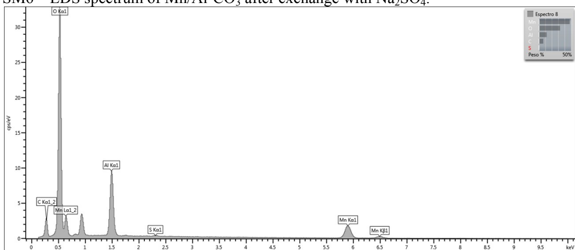
SM6 – EDS spectrum of Mn/Al-CO 3 after exchange with Na 2 SO 4 .
