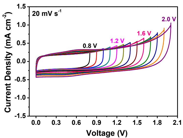
Figure S4. CV curves of the 3D rGO-based SC device with different voltage windows at 20 \text{ mV s}^{-1} .
