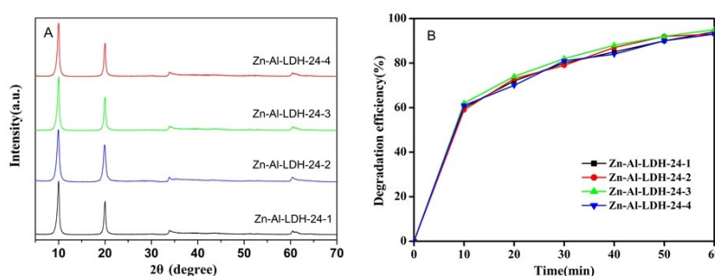
Fig.2 XRD (A) and photocatalytic results (B) of Zn-Al-LDH-24 samples prepared by four repeatability experiments.
