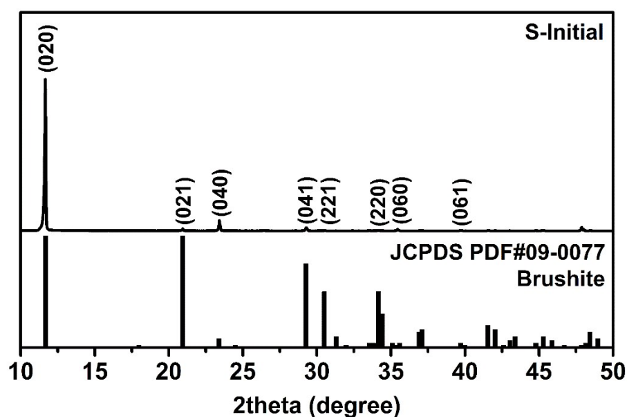
Fig. S1 XRD pattern of the sample obtained in the initial stage (10 min).
