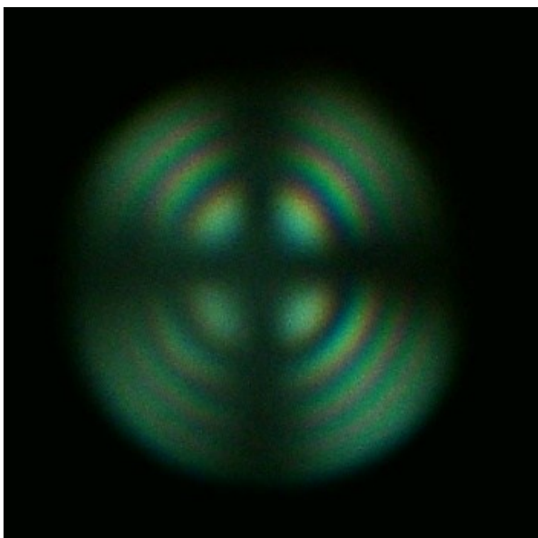
Figure S1. Conoscopic interference figure of \text{Na}_2\text{TiGeO}_5 obtained along the basal pinacoid.
