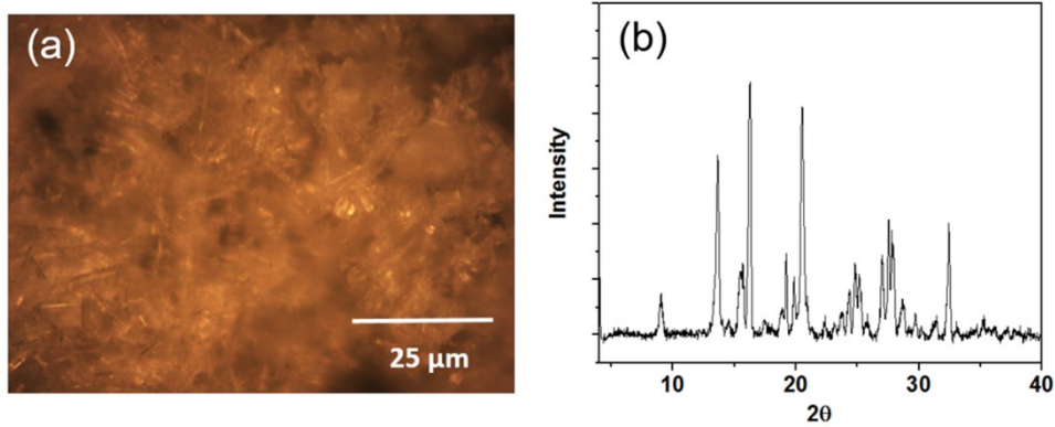
Fig. S2. (a) Microscope image of CBZ prepared in plug flow crystallizer, and (b) the corresponding XRPD
