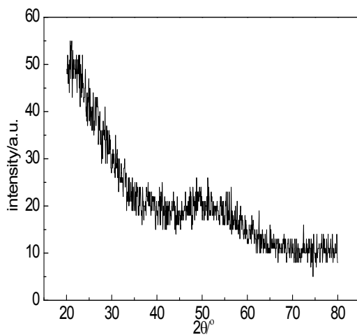
Fig. S1 XRD patterns of amorphous selenium XRD
