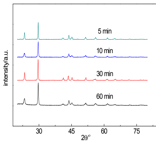
Fig. S2 XRD patterns of nano-selenium at different ultrasonic time
