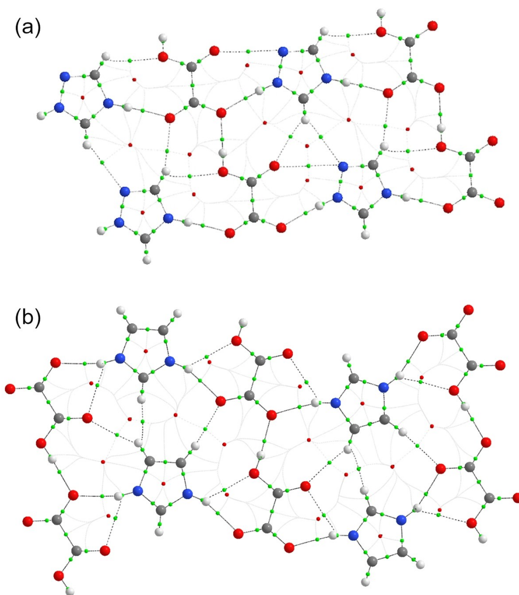
Figure S1 Molecular graphs (QTAIM) of TriOX (a) and ImiOX (b) salts bound through hydrogen bonds. Green circles correspond to bond critical points (BCP).
