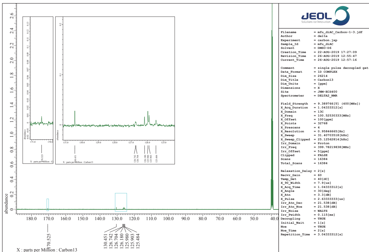
Fig S2 13 C NMR spectra for compound 1
