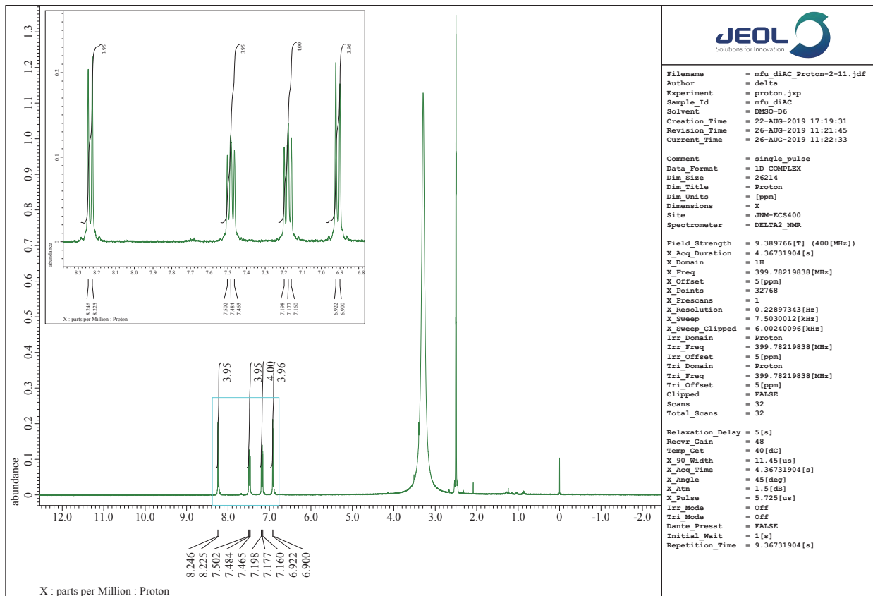
Fig S1 1 H NMR spectra for compound 1
