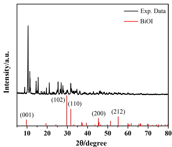
Figure S1, XRD patterns of the products prepared without reaction water.
