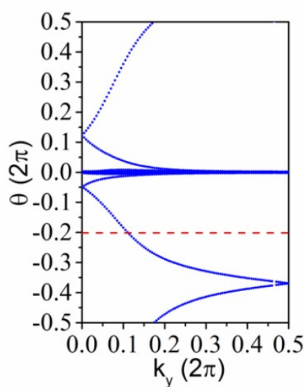
Fig. S1 The evolution of wannier function center of the t -HfC monolayer.
