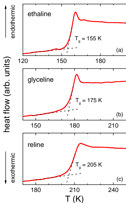
Fig. S1 DSC results on the three DESSs treated in the present work as obtained under heating with 10 K/min.
