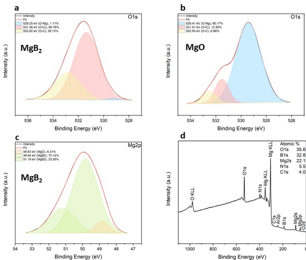
Figure S1: High-resolution O 1s XPS spectra of a) studied \text{MgB}_2 , b) reference \text{MgO} sample c) Mg 2p spectrum of studied \text{MgB}_2 and d) survey XPS spectrum of studied \text{MgB}_2 .
