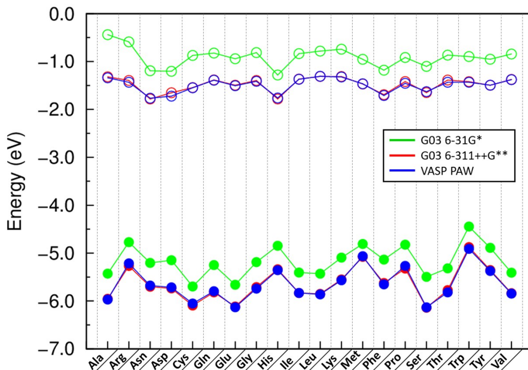
Figure S1. Comparison of calculated HOMO (filled circles) and LUMO (open circles) positions of 20 proteinogenic amino acid molecules with respect to the vacuum level using the plane-wave PAW potential method by VASP and the localized Gaussian basis sets by Gaussian03 [1]. A small (6-31G*) and large converged (6-311++G**) Gaussian basis set are used in the comparison. The VASP results are in excellent agreement with those from the large 6-311++G** basis set.
