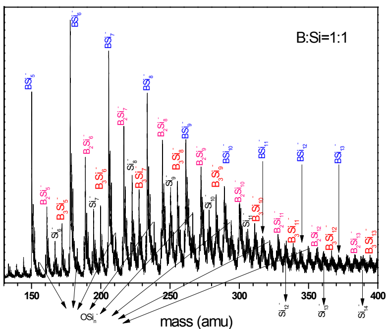
Fig. S1. The typical mass spectrum of B_{1-3}Si_n^- clusters at the sample mole ratio 1:1.
