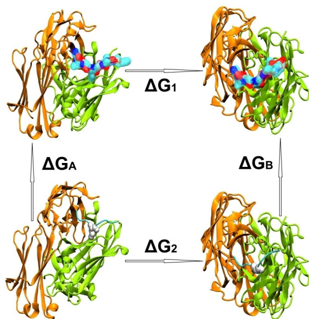
Figure S1. An illustration of the thermodynamic cycle for computing \Delta\Delta G for mutating a residue from Ile to Ala (I515A). Fusion peptide is shown in cyan, while heavy (green) and light (orange) antibody chains are shown in cartoon.
