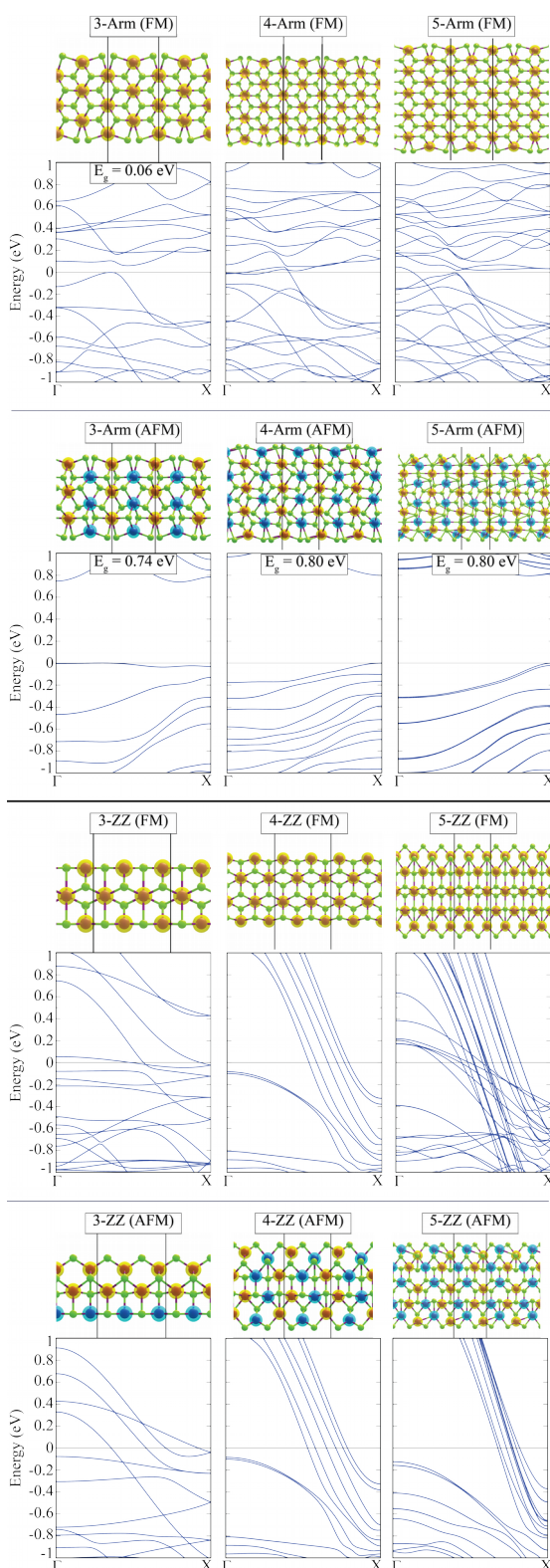
Figure S1 Top views of spin density plots and electronic band structures of nanoribbons of \text{MnSe}_2 .
