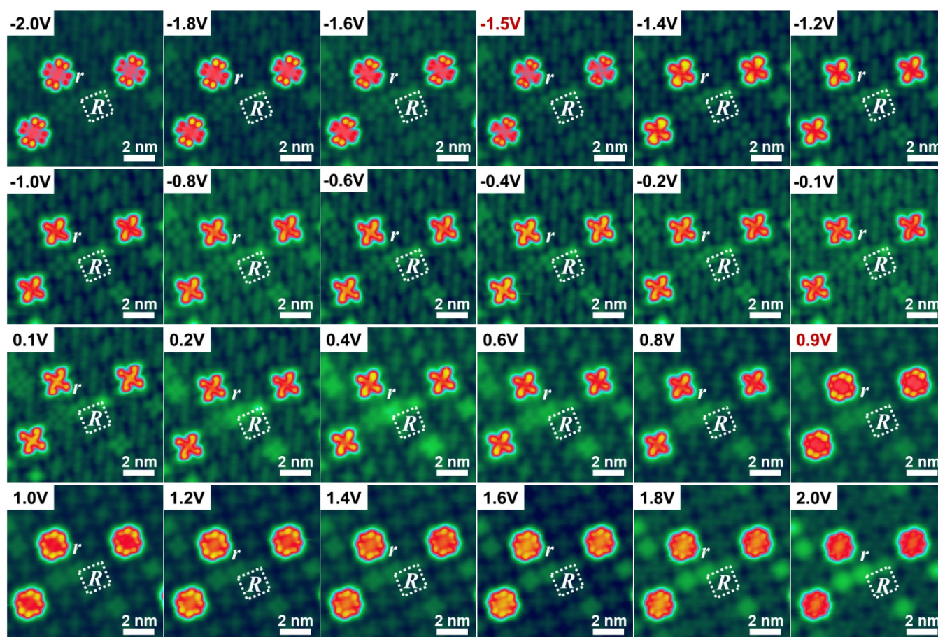
Fig. S1 Constant current STM images of the second-layer TiOPc molecules adsorbed on self-assembled TiOPc monolayer with an Rr chirality at various bias voltages.
