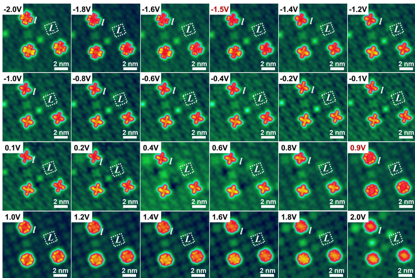
Fig. S2 Constant current STM images of the second-layer TiOPc molecules adsorbed on self-assembled TiOPc monolayer with an L chirality at various bias voltages.
