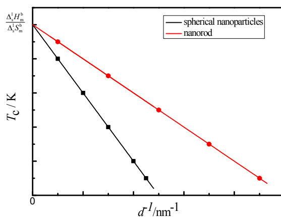
S1 The comparison of melting temperature of nanorods with that of spherical nanoparticles
