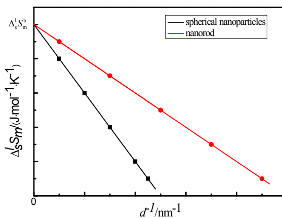
S3 The comparison of melting entropy of nanorods with that of spherical nanoparticles
