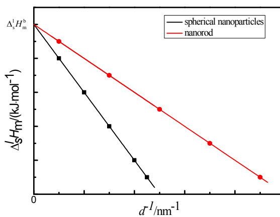
S2 The comparison of melting enthalpy of nanorods with that of spherical nanoparticles
