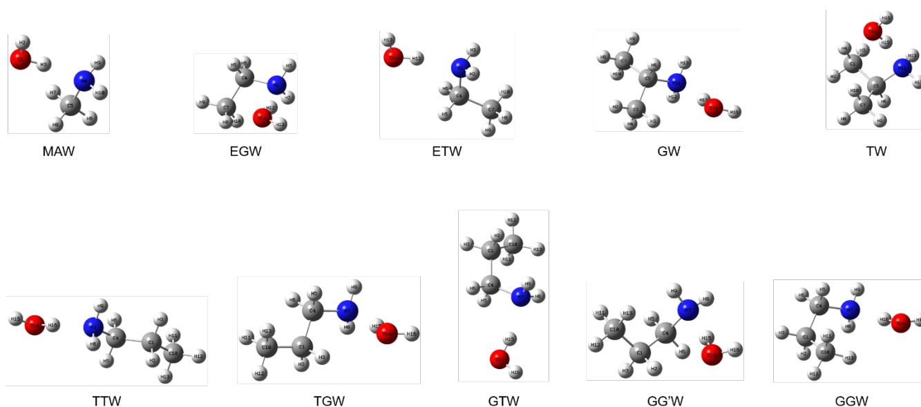
Figure S1. MAW, EGW, ETW, PA-W and IPA-W: atom labelling for Tables S26-S45.
