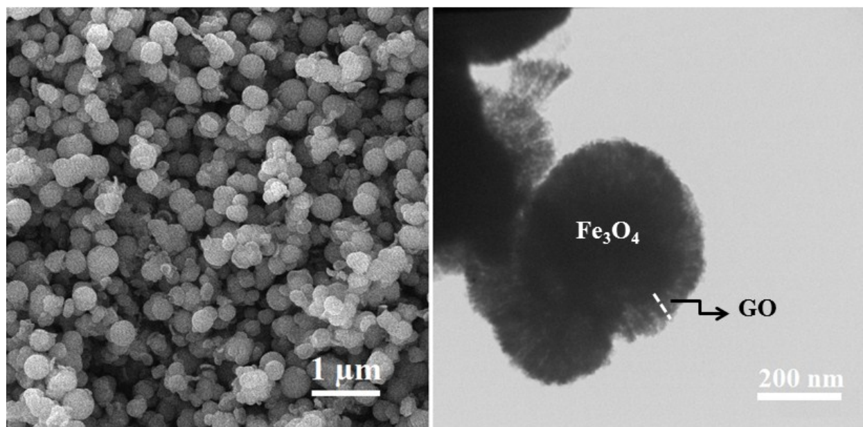
Figure S1. SEM and TEM images of \text{Fe}_3\text{O}_4/\text{GO} sample.
