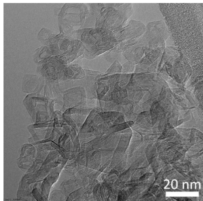
Fig. S5. TEM image of initial BNNPs.
