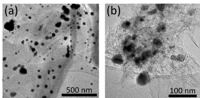
Fig. S2. TEM images of (a) M3_24h and (b) S3_24h samples.
