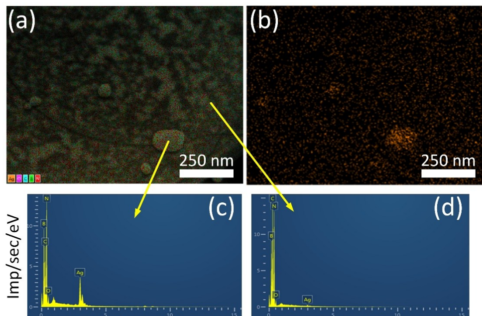
Fig. S1. EDX analysis of the M3_30 sample: electron image with overlaid elemental maps (a), elemental map for Ag (b), and energy spectra (c, d).
