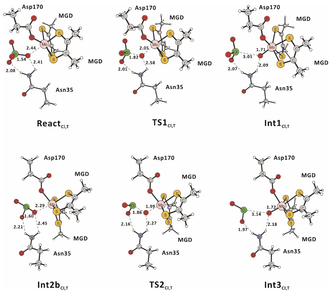
Fig. S4 Optimized structures of stationary points for the PcrAB-catalyzed decomposition of perchlorate in the triplet state. Some important distances are tagged in angstrom (Å). Asterisks indicate the atoms that are fixed at their crystal positions.
