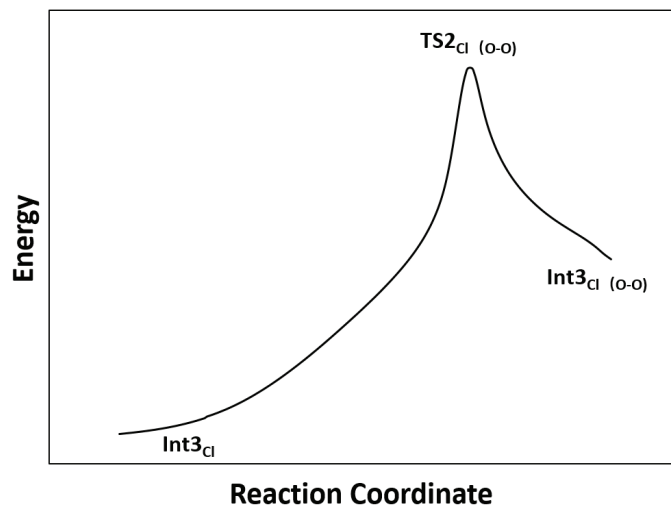
Fig. S7 Schematic potential energy surface obtained by the IRC (intrinsic reaction coordinate) calculations with the TS2 Cl(0-0) structure as the starting point.
