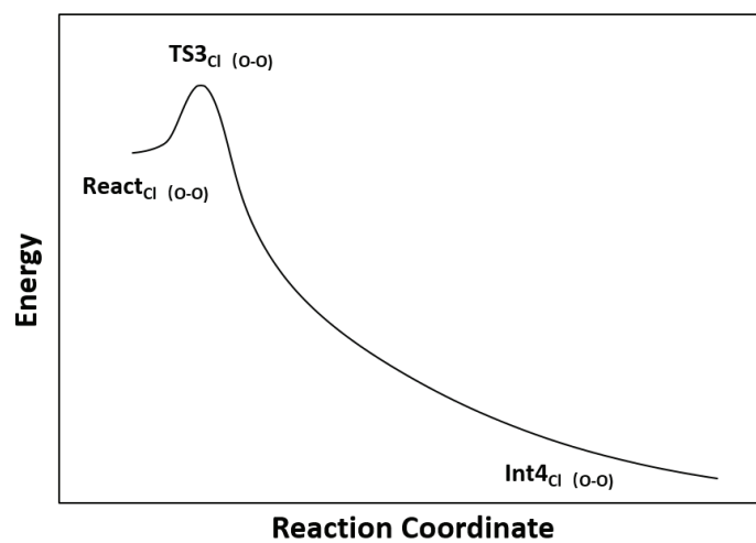
Fig. S8 Schematic potential energy surface obtained by the IRC (intrinsic reaction coordinate) calculations with the TS3 Cl(0-0) structure as the starting point.
