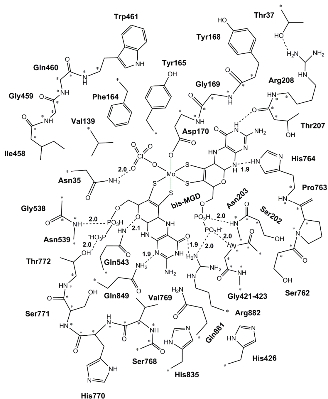
Fig. S2 A bigger model (537 atoms) of the PcrAB active site used in this work. For clarity, 2-D schematic structure is shown. Asterisks indicate the atoms which are fixed to their X-ray positions. The distances optimized are in angstroms (Å).
