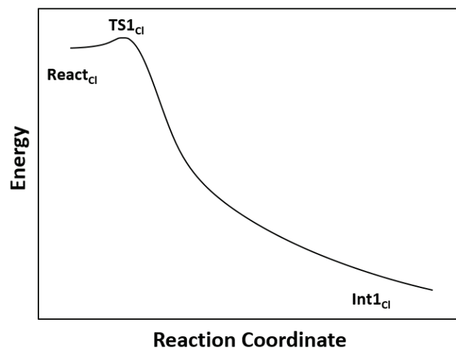
Fig. S3 Schematic potential energy surface obtained by the IRC (intrinsic reaction coordinate) calculations with the TS1 cl structure as the starting point.
