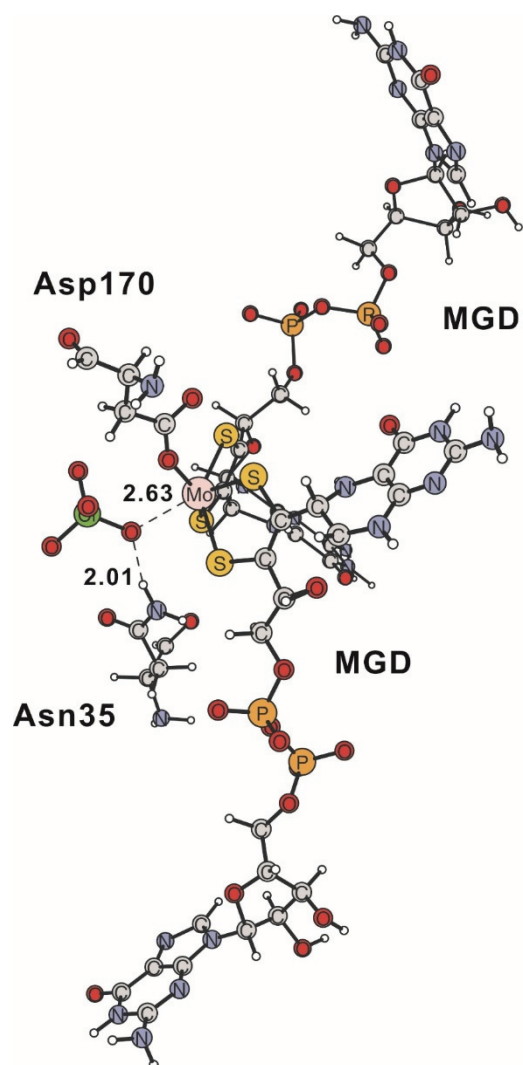
Fig. S1 The binding of perchlorate in the PcrAB active site predicted by the docking simulation. Some important distances are tagged in angstrom (Å).
