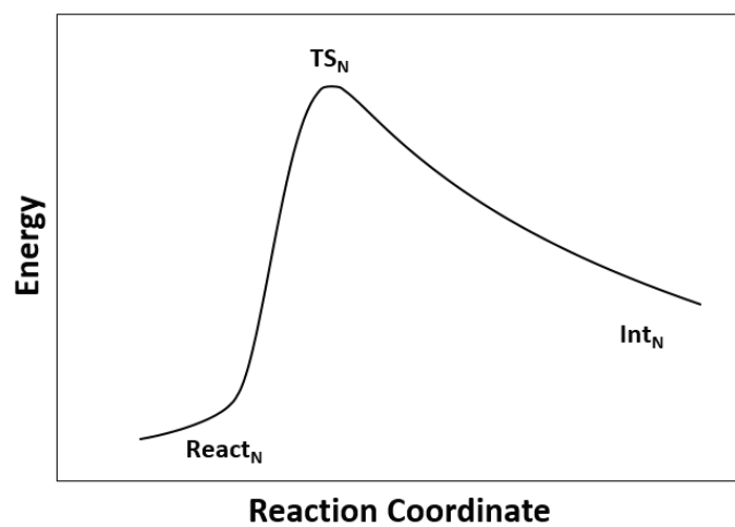
Fig. S9 Schematic potential energy surface obtained by the IRC (intrinsic reaction coordinate) calculations with the TS N structure as the starting point.
