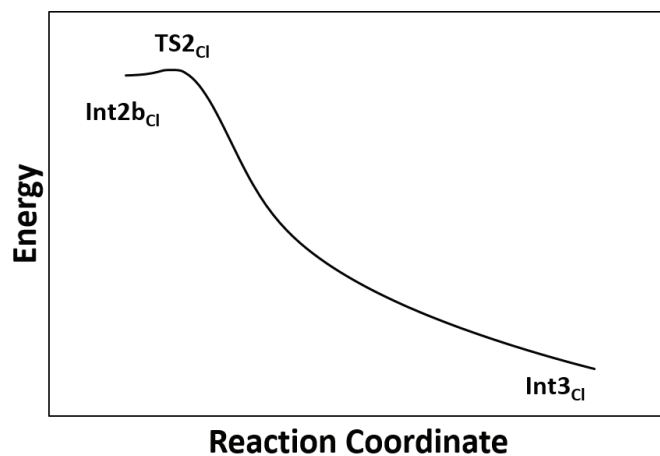
Fig. S5 Schematic potential energy surface obtained by the IRC (intrinsic reaction coordinate) calculations with the TS2 Cl structure as the starting point.
