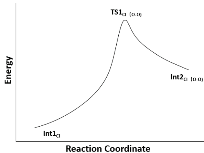
Fig. S6 Schematic potential energy surface obtained by the IRC (intrinsic reaction coordinate) calculations with the TS1 Cl(0-0) structure as the starting point.
