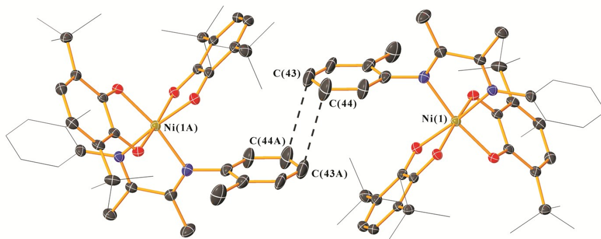
SI Figure 1. Intermolecular contacts between adjacent molecules in 1.
