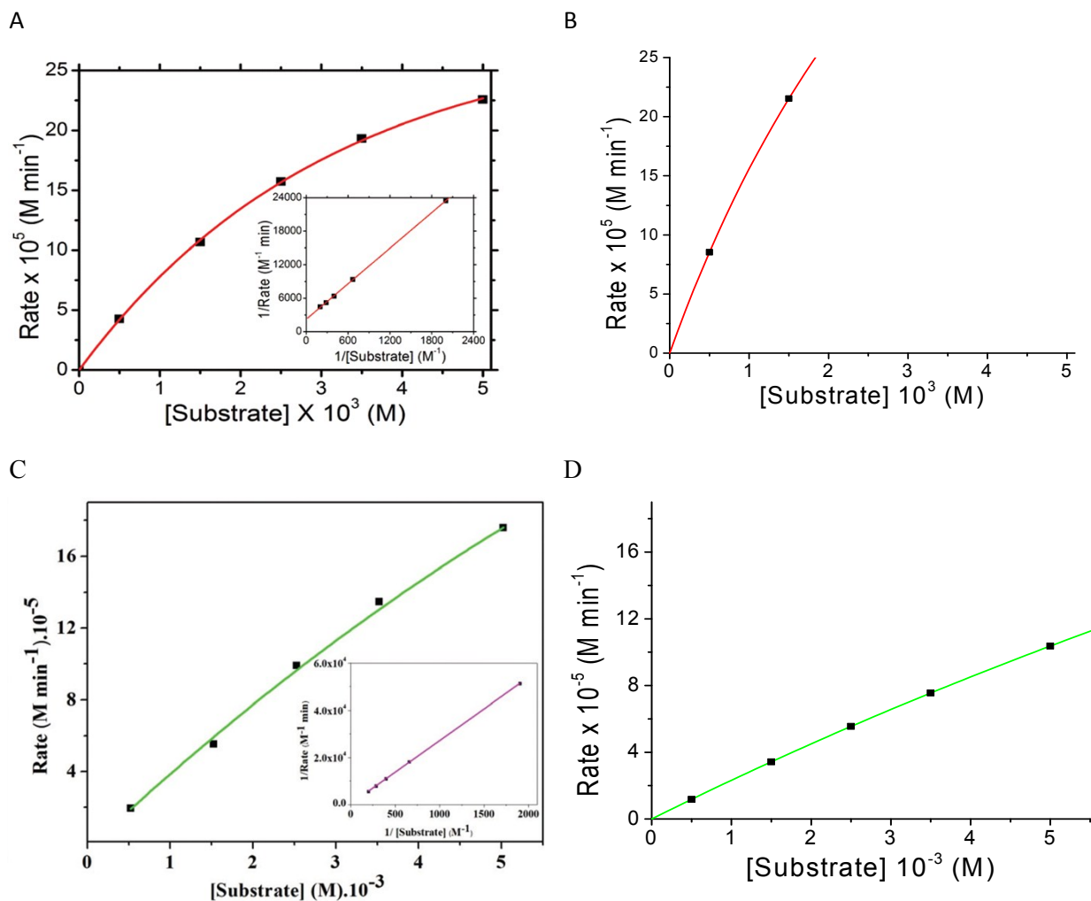
Figure S1. Reported and simulated plots of Rate vs [Substrate]. A and C are plots reported in 1 and 2 , respectively. B and D were generated from the kinetic parameters reported in the same articles, we kept the same scale in y to facilitate the comparison.
