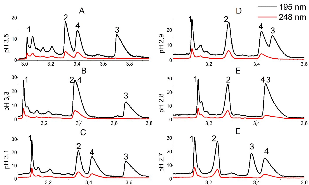
Fig. S1. The CZE separations of [\text{Rh}_y(\text{OH})_m(\text{H}_2\text{O})_z]^{3y-m} complexes within pH range from 3.5 to 2.7
