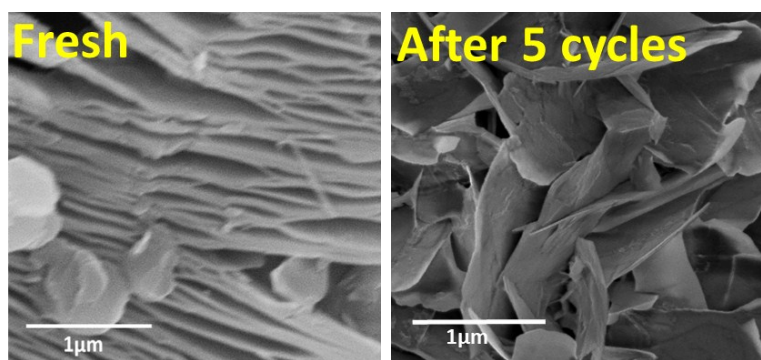
Fig. S2 SEM images of unloaded MXene (Pristine) and Regenerated MXene after 5 cycles.
