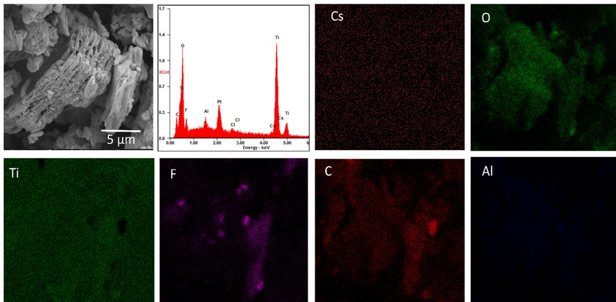
Fig. S1 SEM image, EDS spectra and corresponding elemental mapping images of Cs, O, Ti, F, C and Al, respectively from Cs Loaded MXene.
